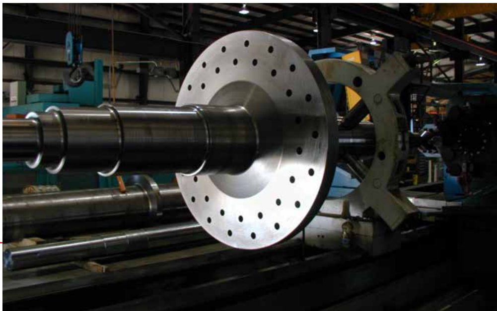
Drilling Flange holes with live tooling CNC lathe
